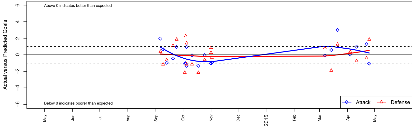
FC Nova SuperNova Black B03 Dots are actual minus expected GF (blue circles) and GA (red triangles). Blue line is smoothed change in attack strength. Red is smoothed change in defense strength.
